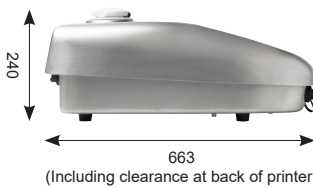
Side Elevation
